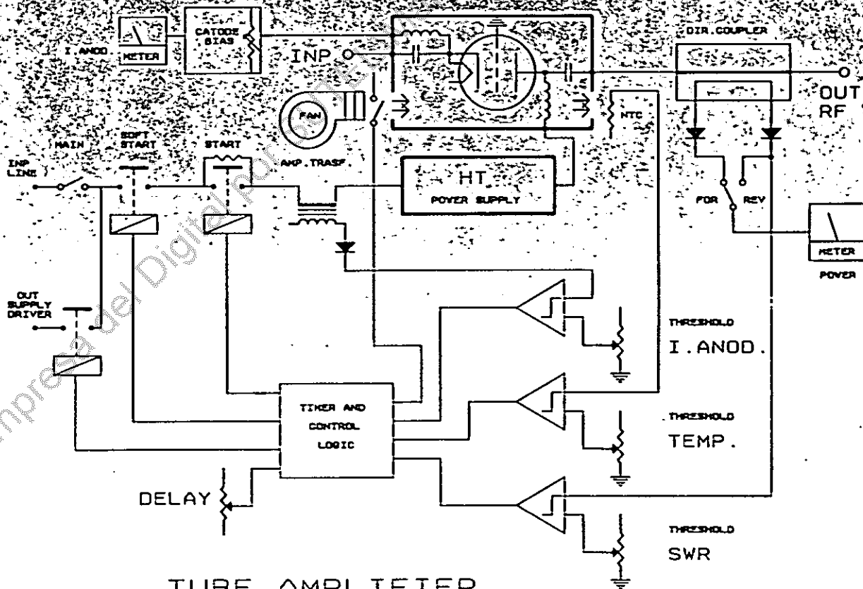
TUBE AMPLIFIER
