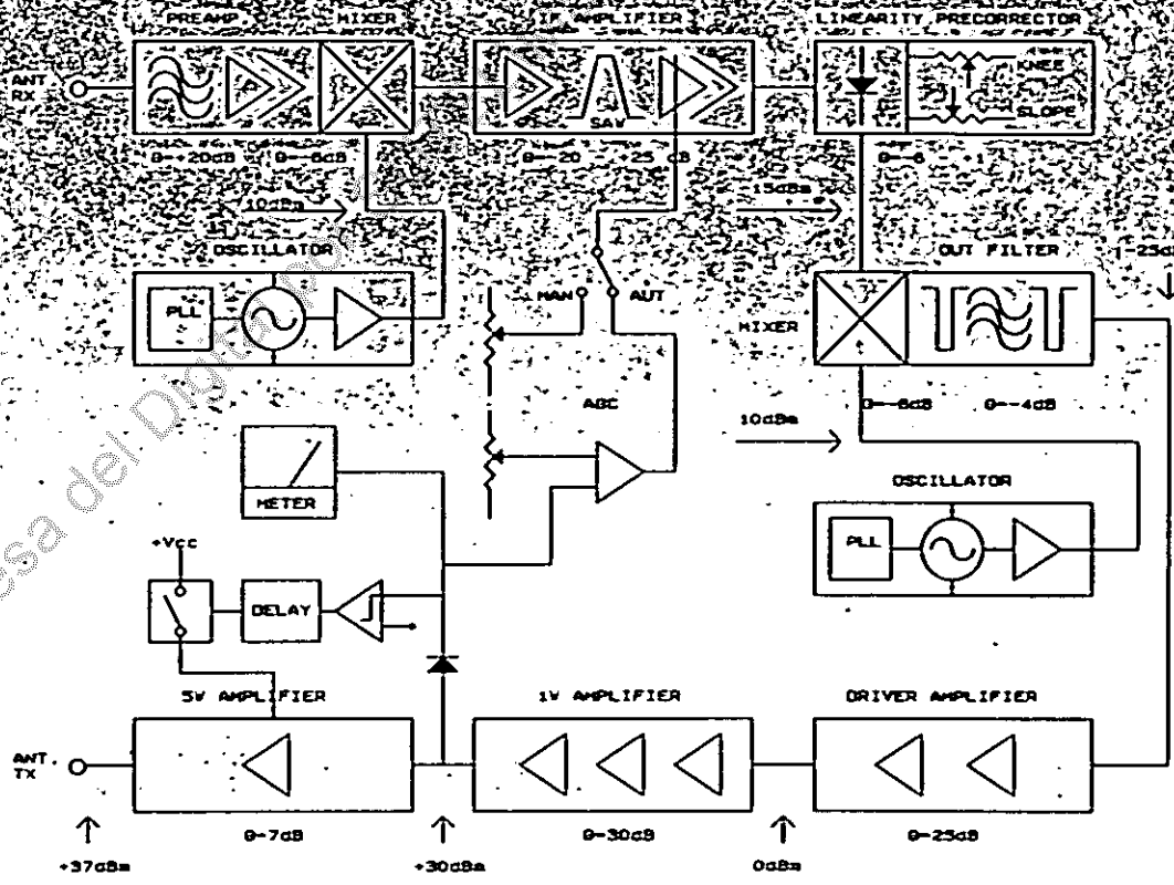
TV TRANSPOSER
